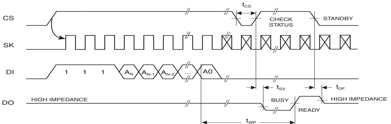
Figure 8. ERASE Timing
