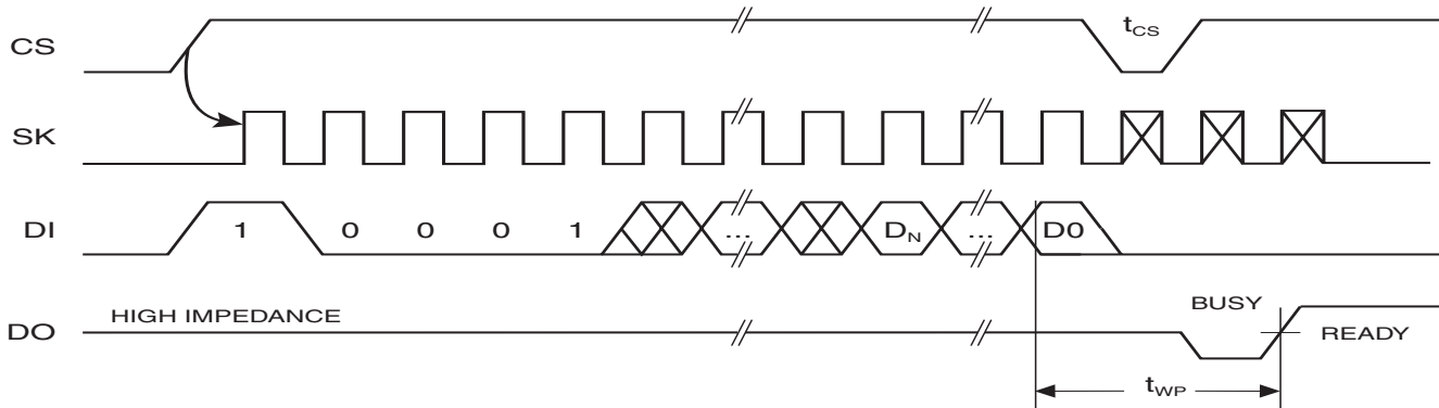
Figure 7. WRAL Timing (1),(2)
