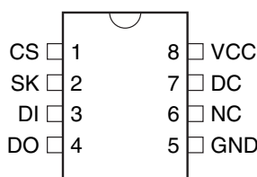
8-lead SOIC
