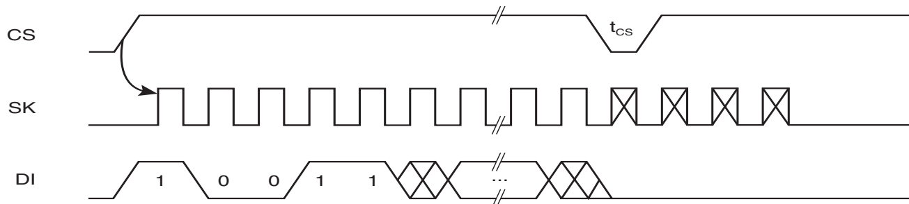
Figure 4. EWEN Timing 1
