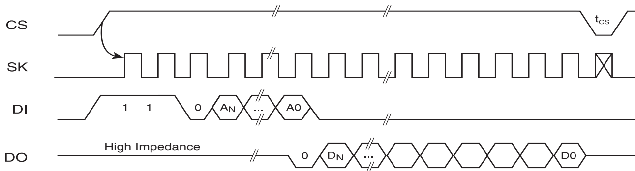
Figure 3. READ Timing
