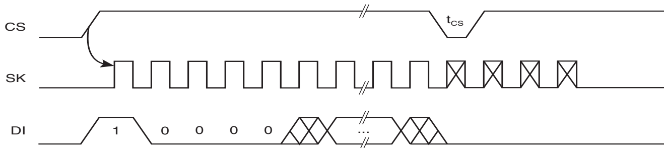
Figure 5. EWDS Timing 1
